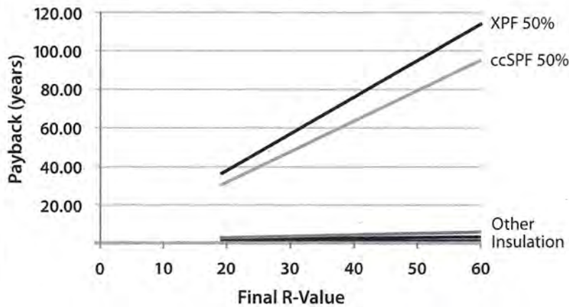
Figure 1. Lifetime GWP Payback XPS & SPF
